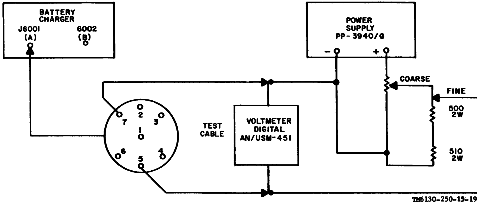
Figure 6-2. Test setup for adjusting battery discharger cutoff circuit.
