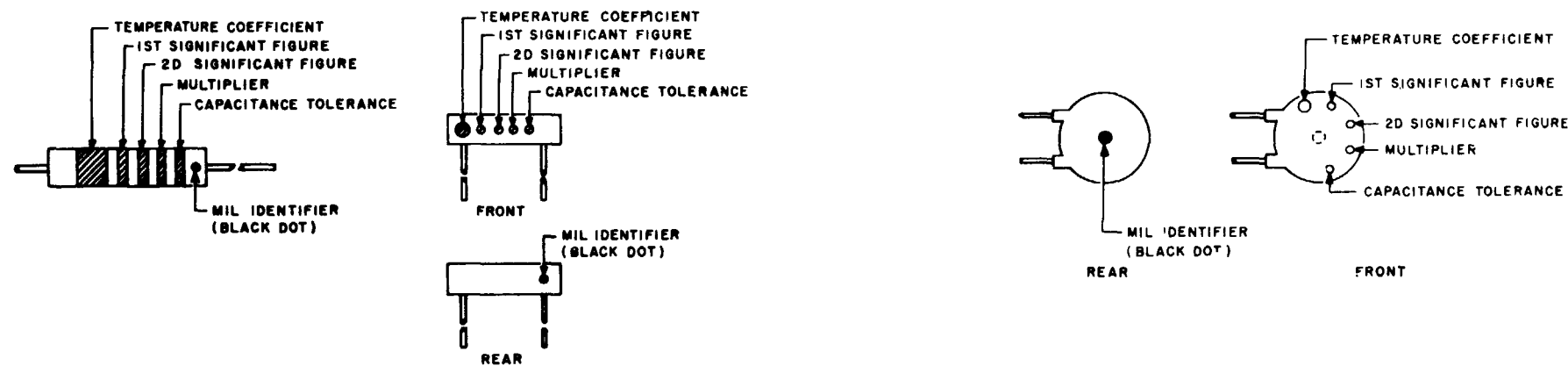
Figure 9-2. MIL-STD capacitor color code markings.
