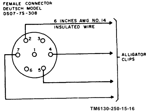
Figure 5-6. Test cable construction diagram.
