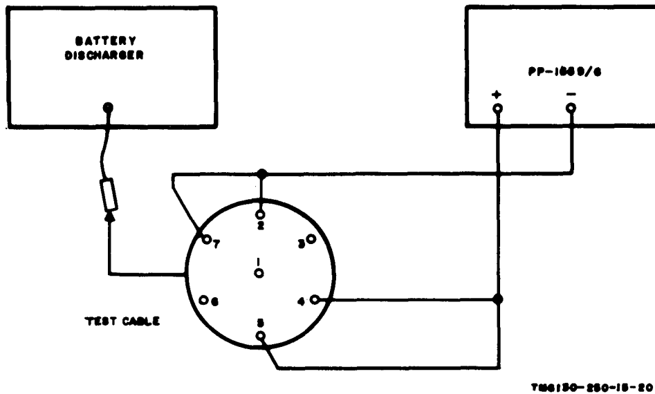
Figure 6-3. Test setup for adjusting battery discharger cutoff circuit.
