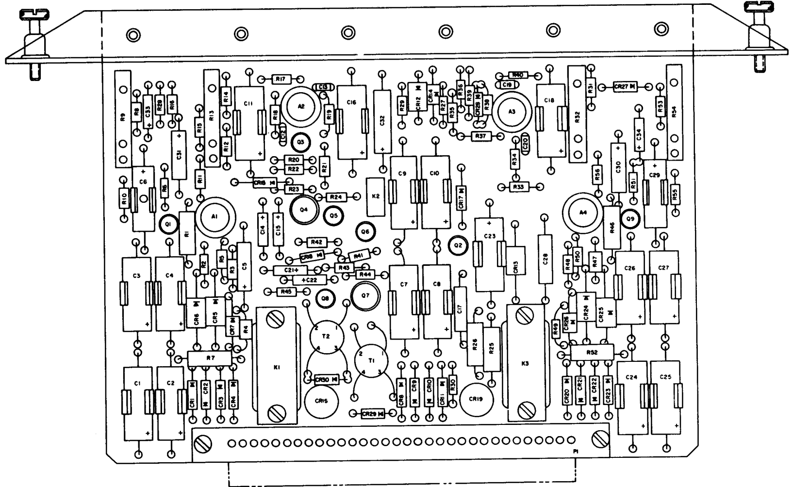
Figure 9-3. Battery charger printed circuit board component locations.
