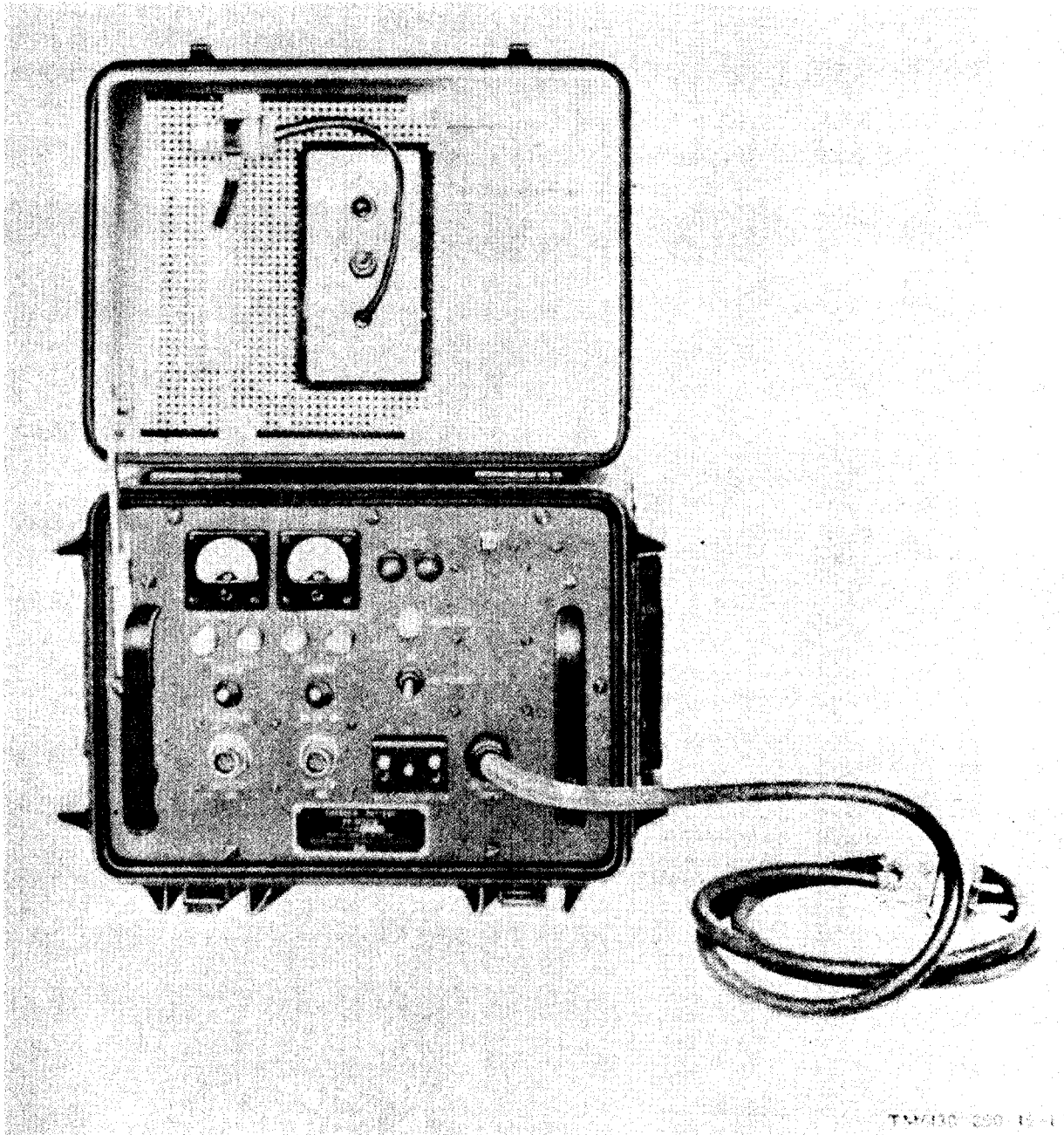
Figure 1-1. Charger, Battery PP-4127/U, cover open.
