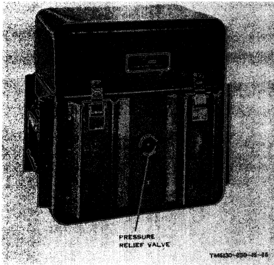
Figure 1-2. Charger, Battery PP-4127/U, cover closed.
