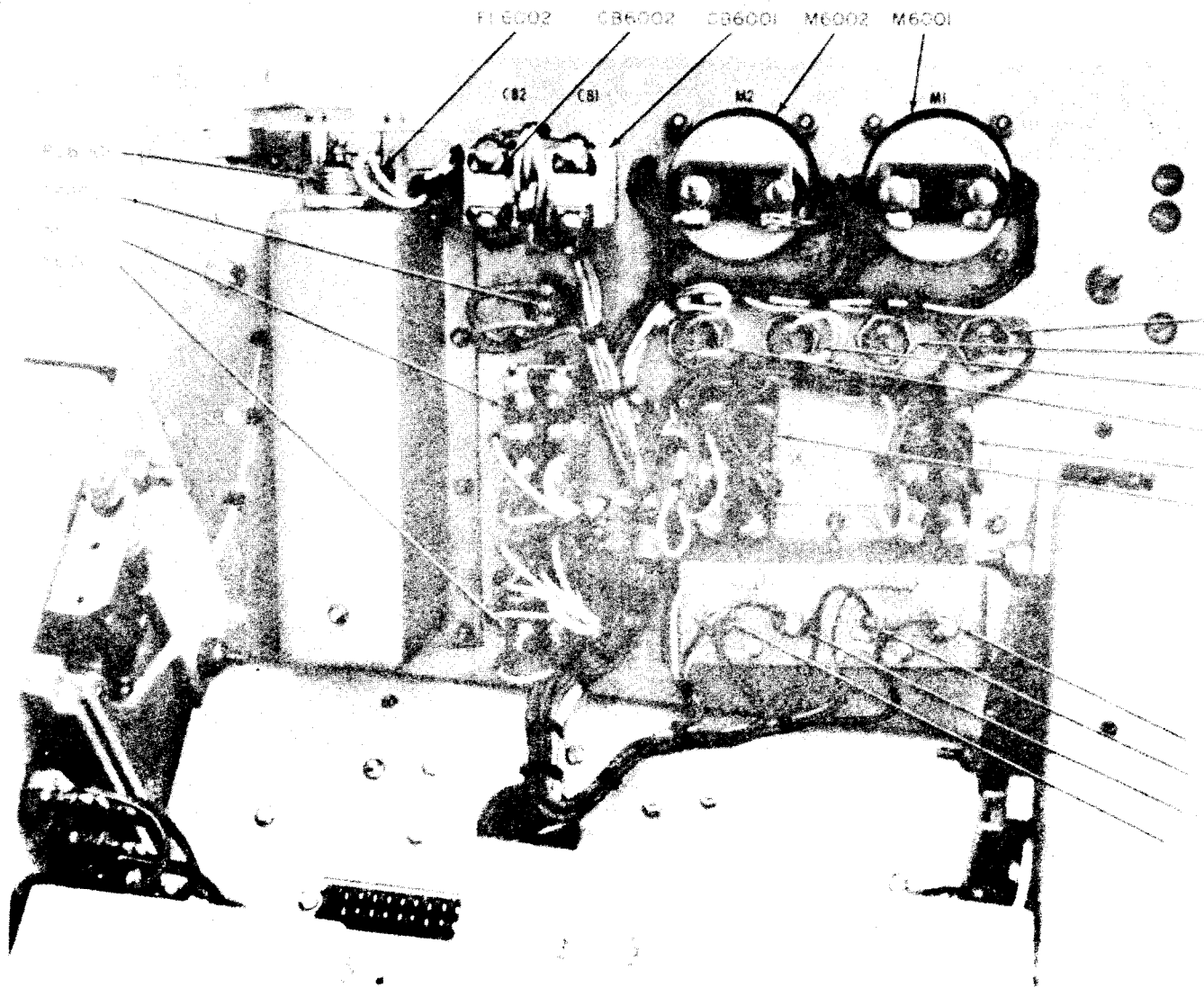
Figure 5-2. Battery charger component locations, rear of front panel.
