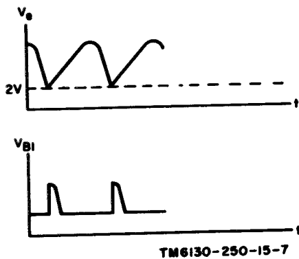
Figure 4-3. Basic UJT multivibrator circuit
