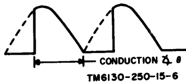
Figure 4-3. Voltage at cathode of SCR.
